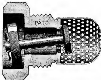
Fig. 3020. Sectional View. GOLD'S GRAVITY RELIEF TRAP.
